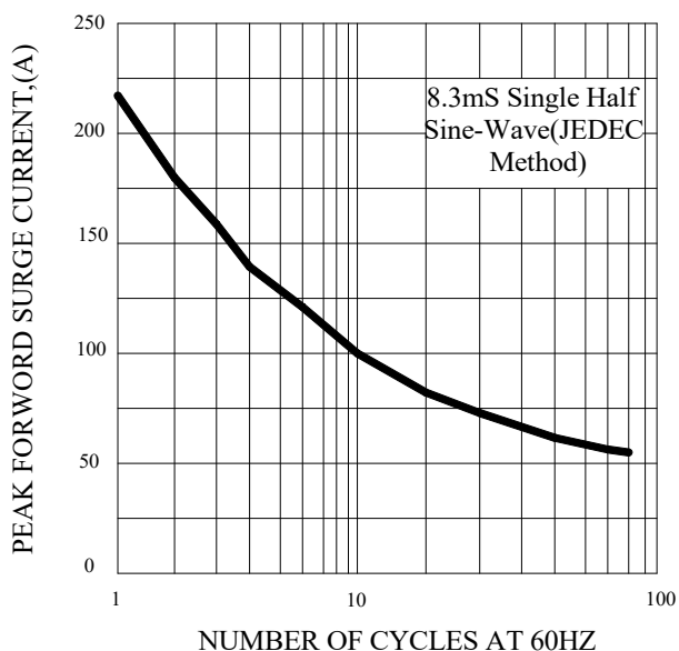
FIG.3-MAXIMUM NON-REPEITIVE FORWARD SURGE CURRENT
